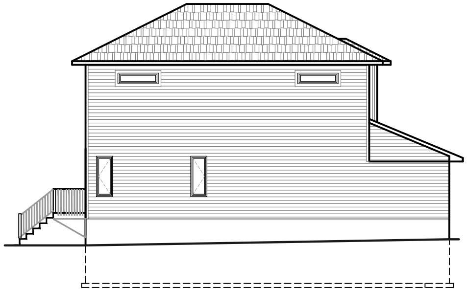
LEFT ELEVATION-ROCKPORT 33
