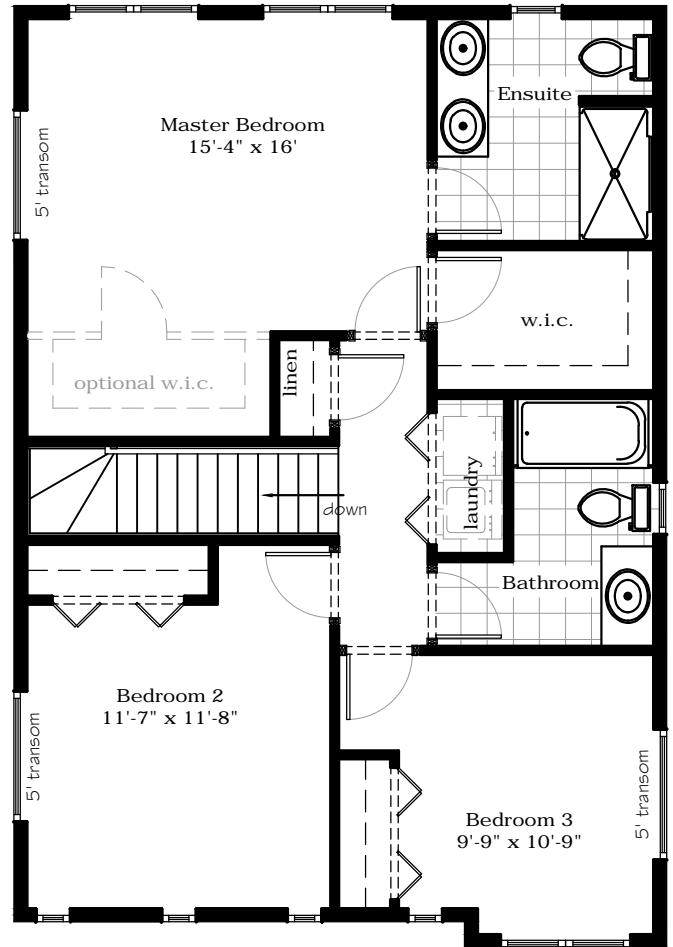
Second Floor Plan-885 sf
